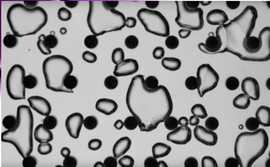
Air-water flow through a pin-fin array designed to break up large bubbles and generate more interface area.
